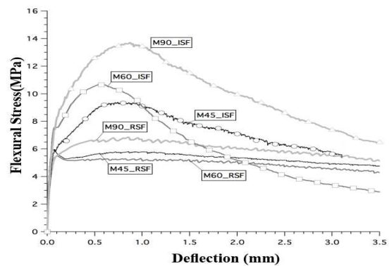
Figure 8. Comparison of the flexural behaviour of ISFRC and RSFRC.
