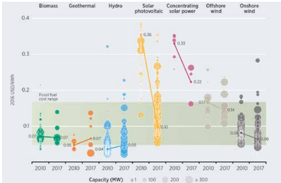
Figure 1: Levelised cost of electricity by project and weighted average by technology, 2010 and 2017
