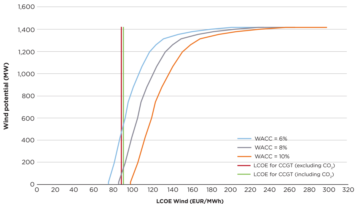
Figure 4.29: Cost-competitive wind potential in Slovenia in 2016
