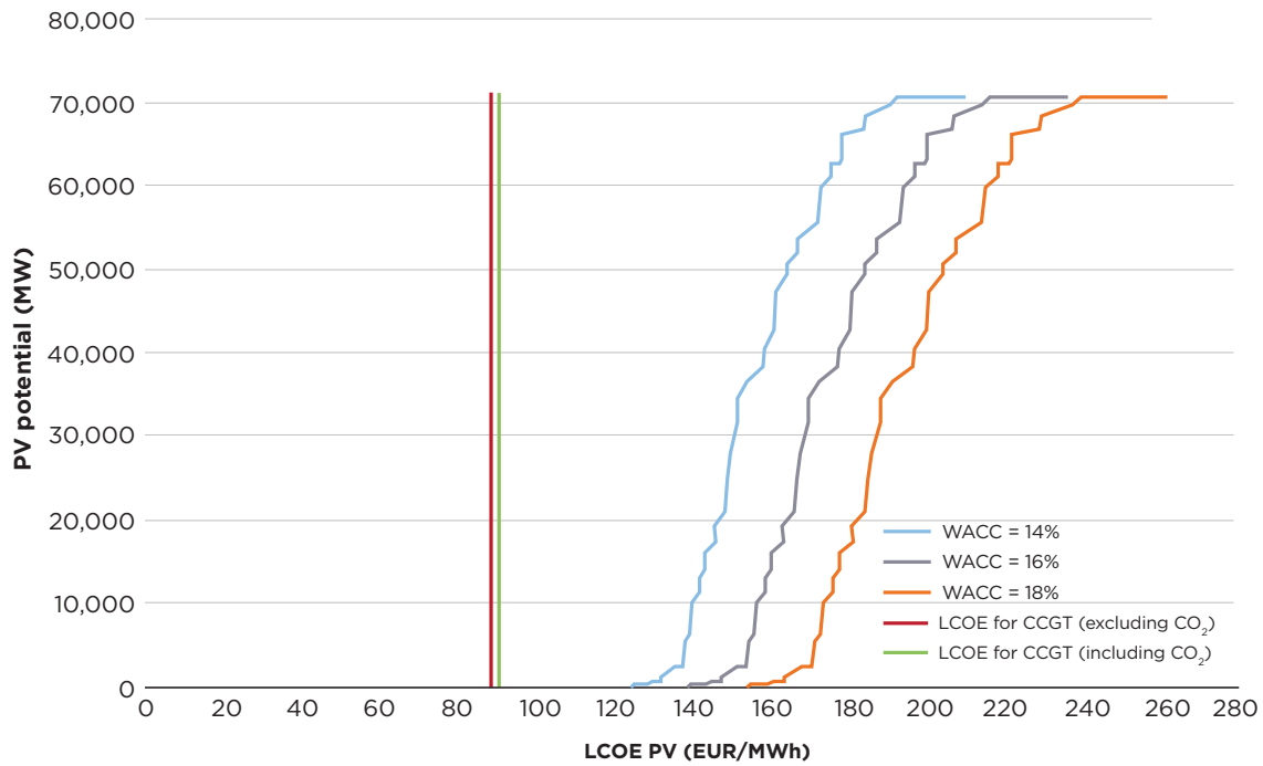
Figure 4.34: Cost-competitive solar PV potential in Ukraine in 2016
