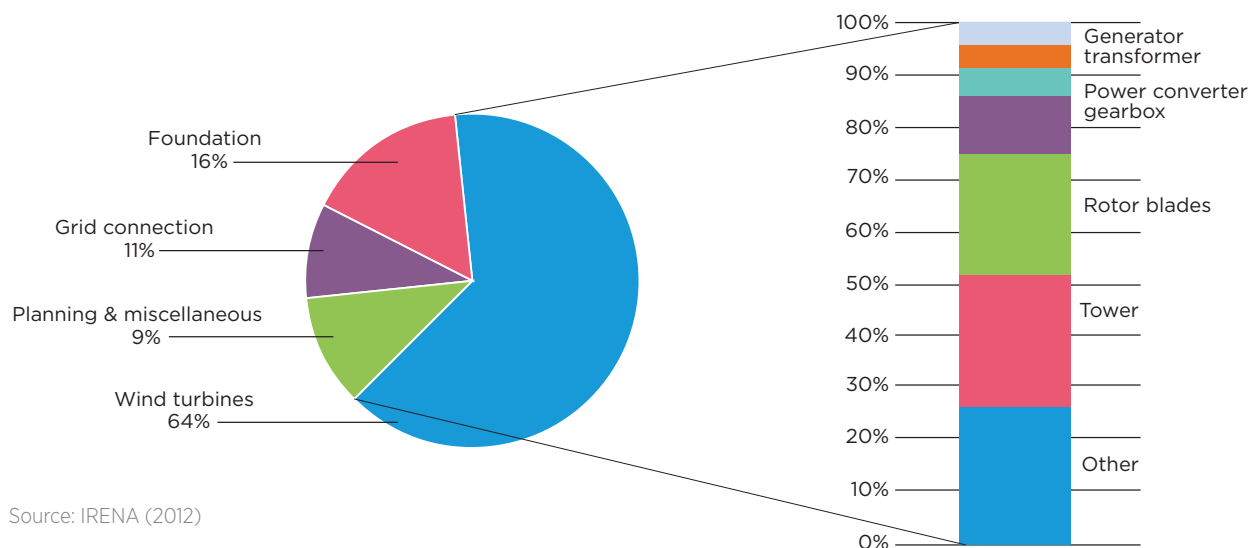
Figure 7.3: Capital cost breakdown for a typical onshore wind power system and turbine
