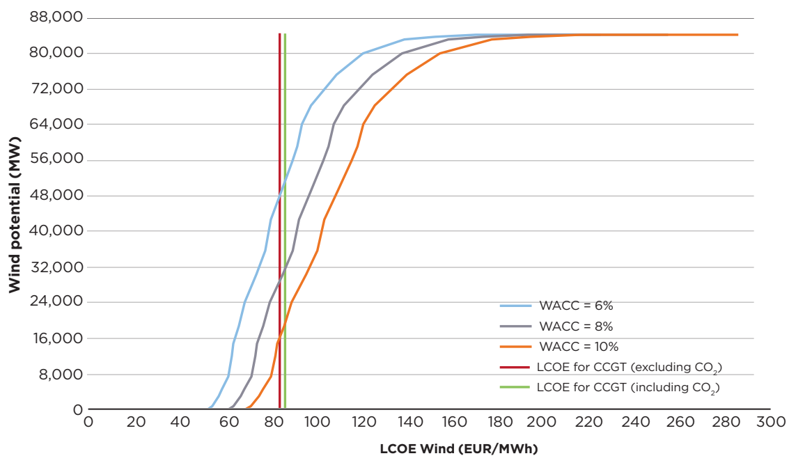
Figure 4.23: Cost-competitive wind potential in Romania in 2016
