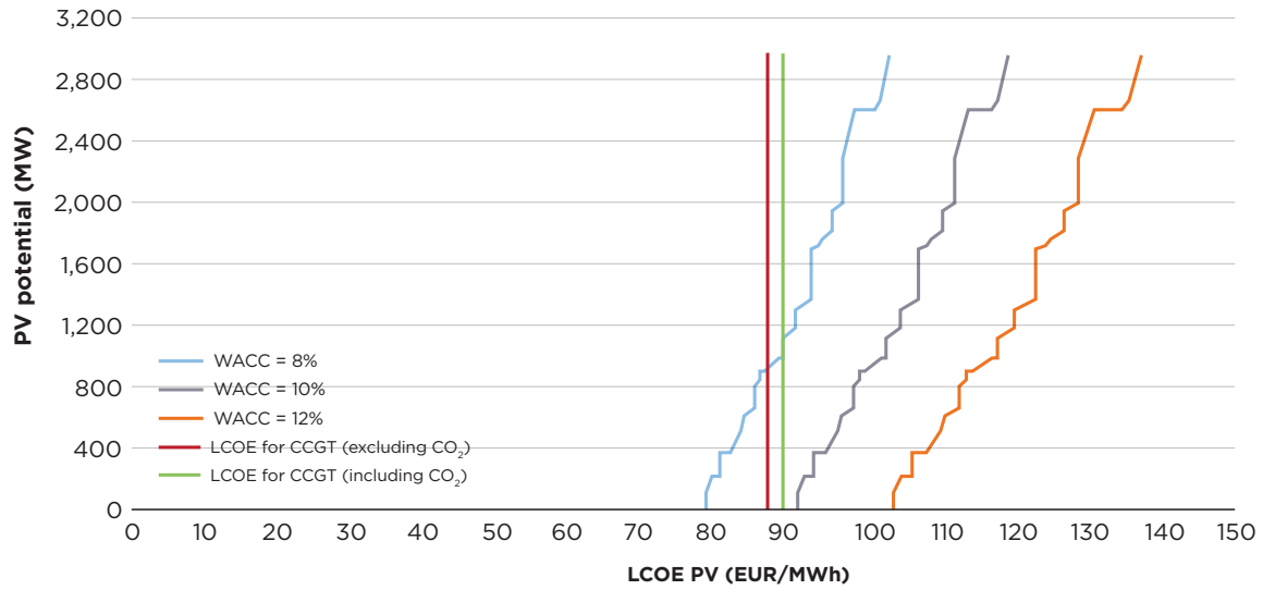
Figure 4.4: Cost-competitive solar PV potential in Bosnia and Herzegovina in 2016
