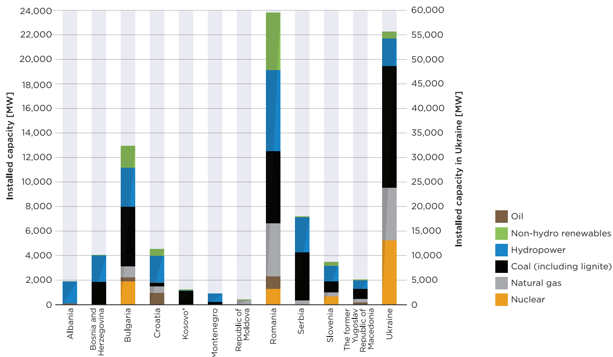
Figure 1.1: Power systems of SEE in 2015 8
