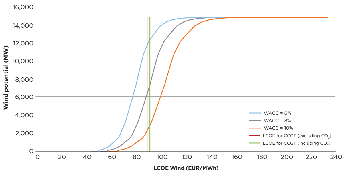
Figure 4.11: Cost-competitive wind potential in Croatia in 2016
