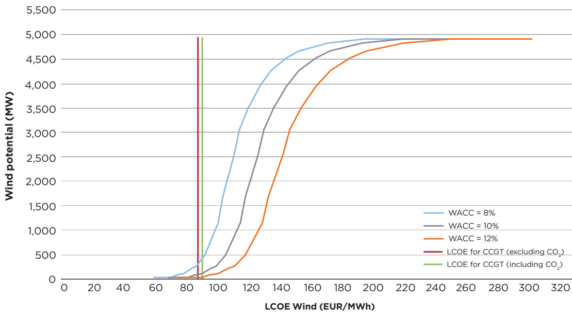
Figure 4.32: Cost-competitive wind potential in the former Yugoslav Republic of Macedonia in 2016
