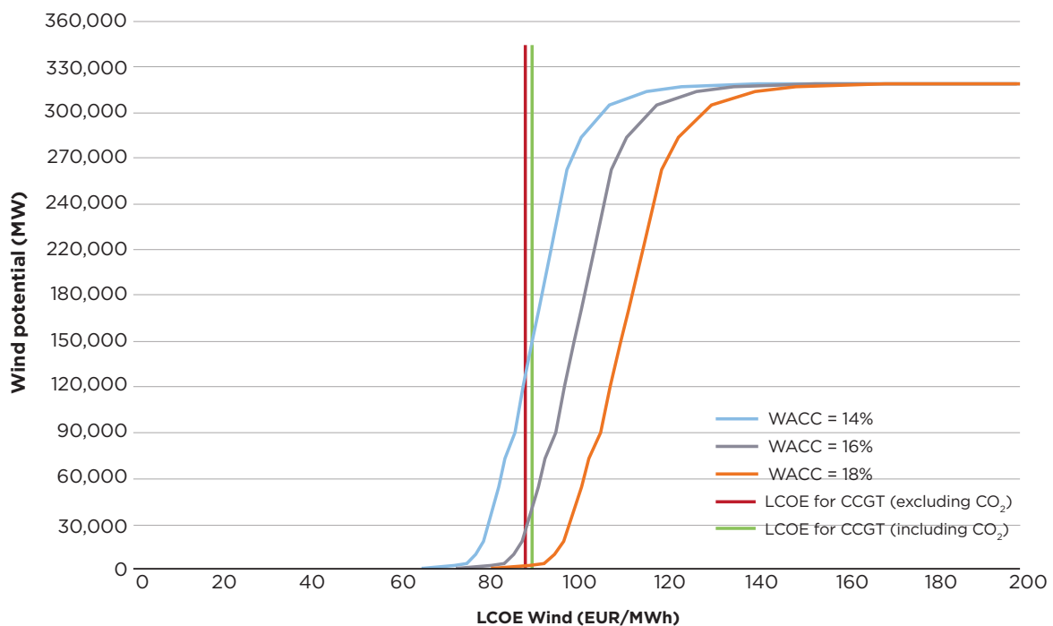
Figure 4.35: Cost-competitive wind potential in Ukraine in 2016
