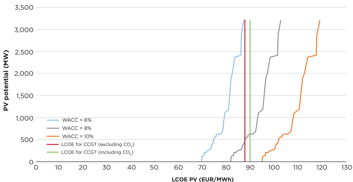
Figure 4.10: Cost-competitive solar PV potential in Croatia in 2016
