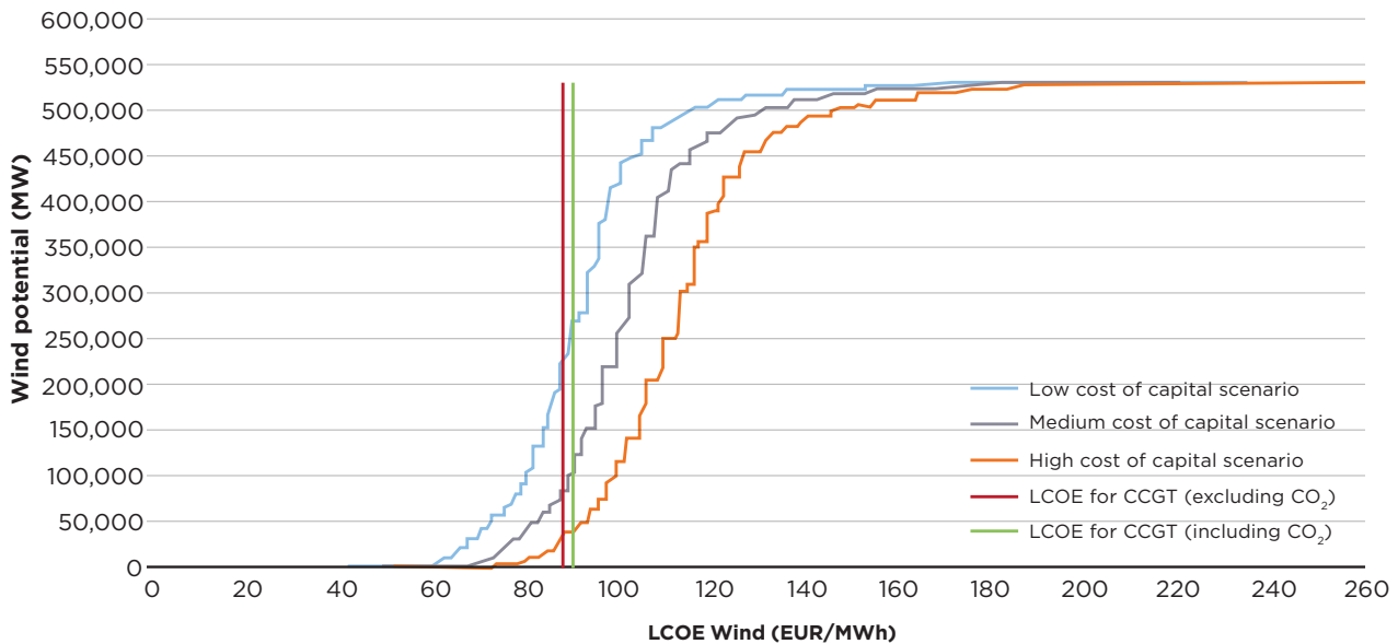
Figure 3.7 Cost-competitive wind potential in SEE in 2016
