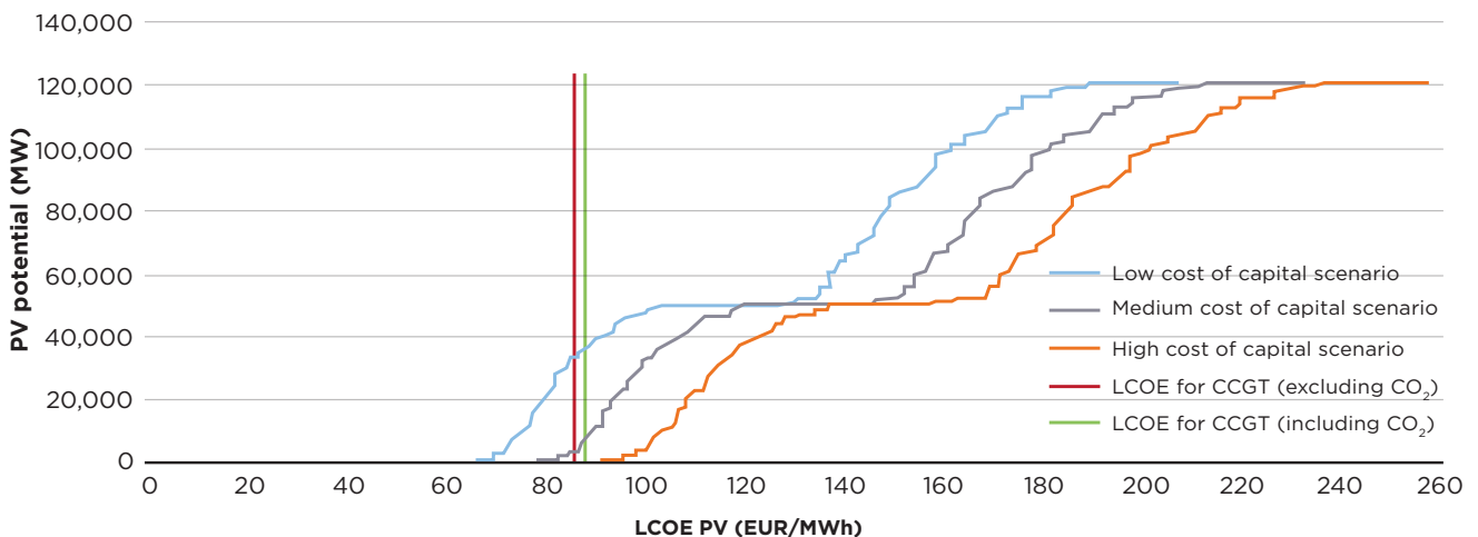
Figure 3.8 Cost-competitive solar PV potential in SEE in 2016
