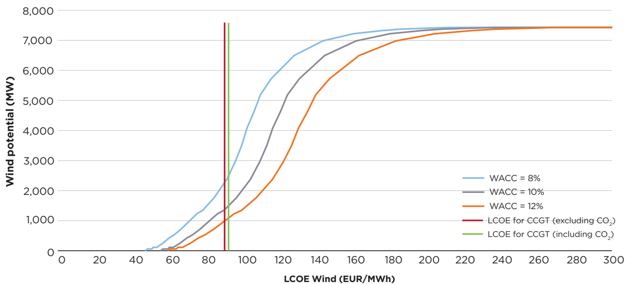
Figure 4.2: Cost-competitive wind potential in Albania in 2016
