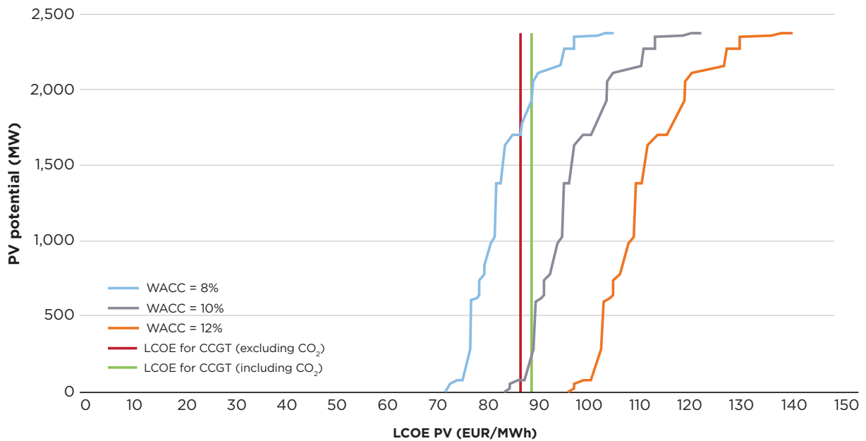
Figure 4.1: Cost-competitive solar PV potential in Albania in 2016
