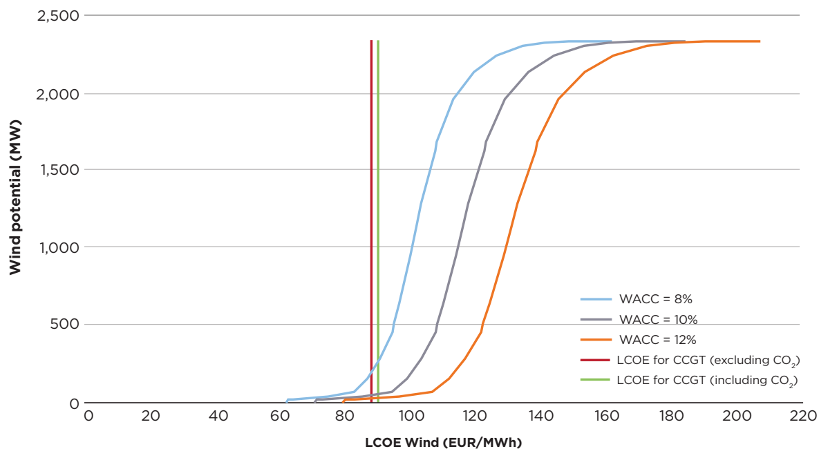
Figure 4.14: Cost-competitive wind potential in Kosovo* in 2016
