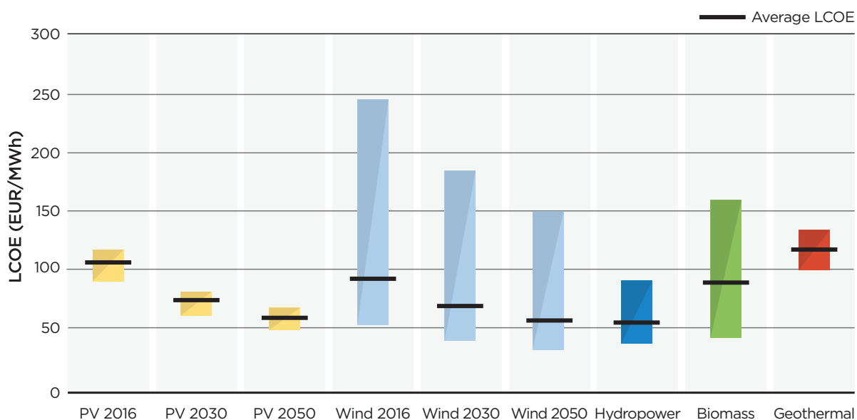
Figure 4.18: LCOE ranges and weighted averages of renewable energy technologies in Montenegro (medium cost of capital)
