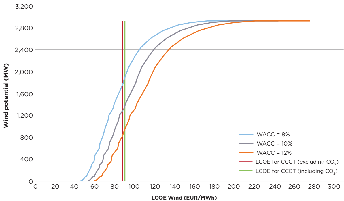
Figure 4.17: Cost-competitive wind potential in Montenegro in 2016
