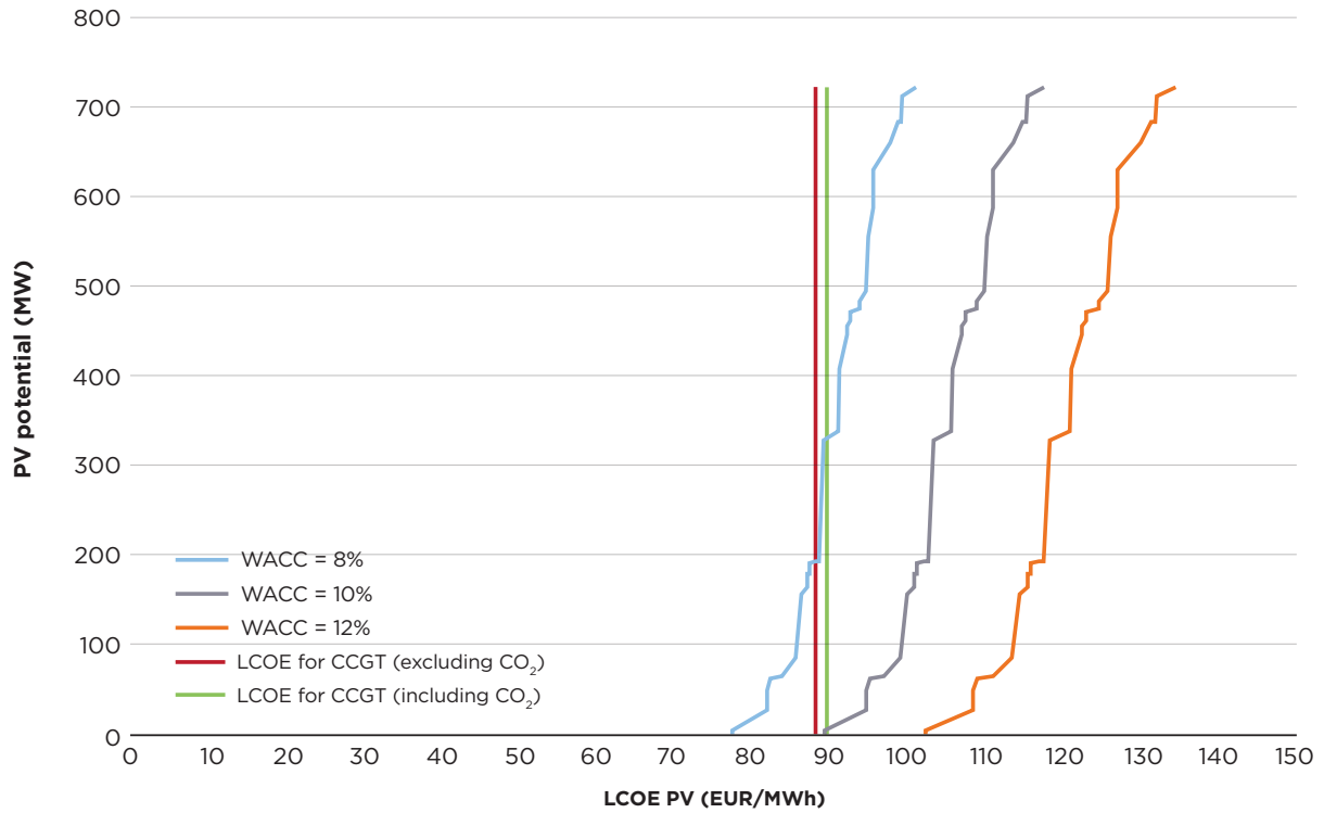
Figure 4.16: Cost-competitive solar PV potential in Montenegro in 2016
