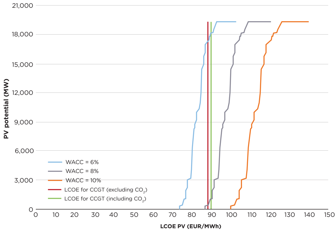
Figure 4.22: Cost-competitive solar PV potential in Romania in 2016
