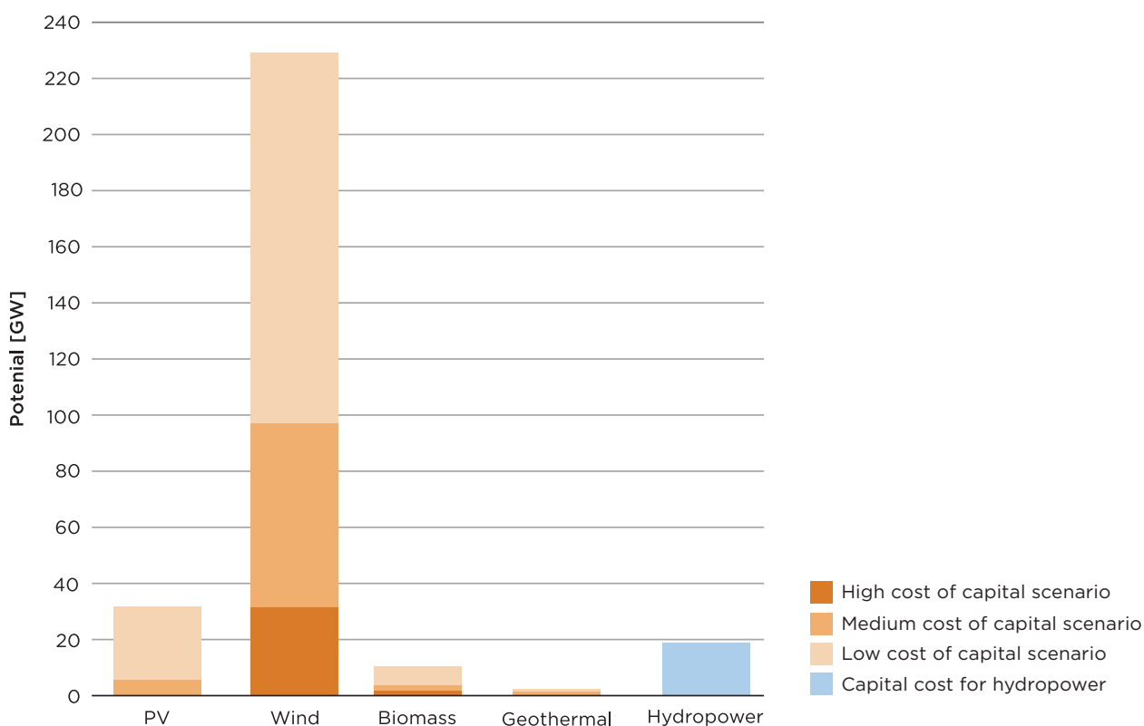
Figure 3.4: Cumulative additional cost-competitive renewable power potential for SEE in 2016 (292.7 GW)
