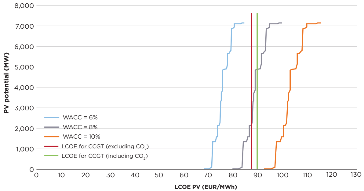
Figure 4.7: Cost-competitive solar PV potential in Bulgaria in 2016
