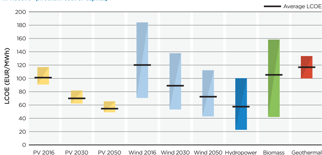
Figure 4.15: LCOE ranges and weighted averages of renewable energy technologies in Kosovo* (medium cost of capital)
